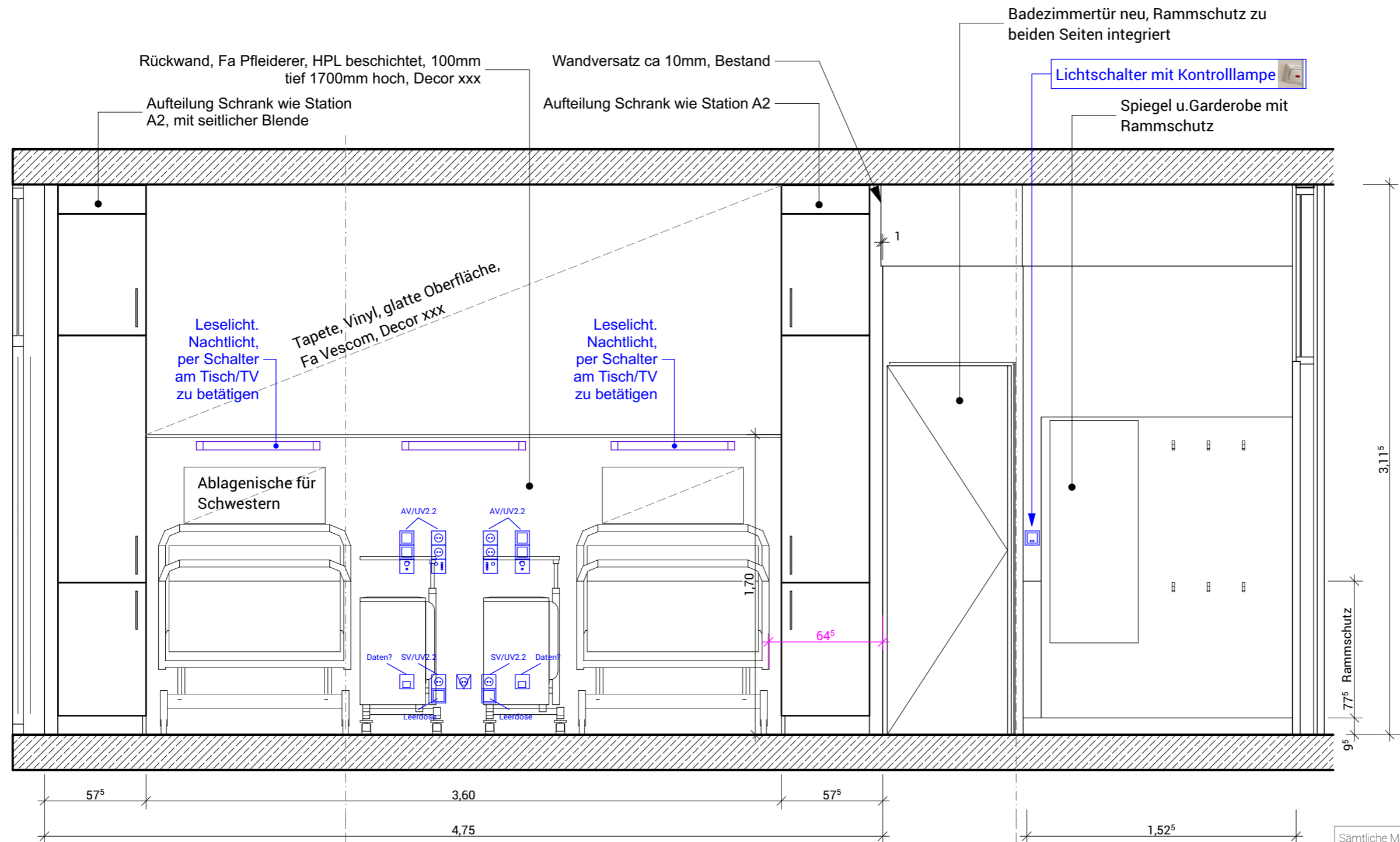
Referenz Elektroanschlüsse Kopfende Patientenzimmer Station A2
