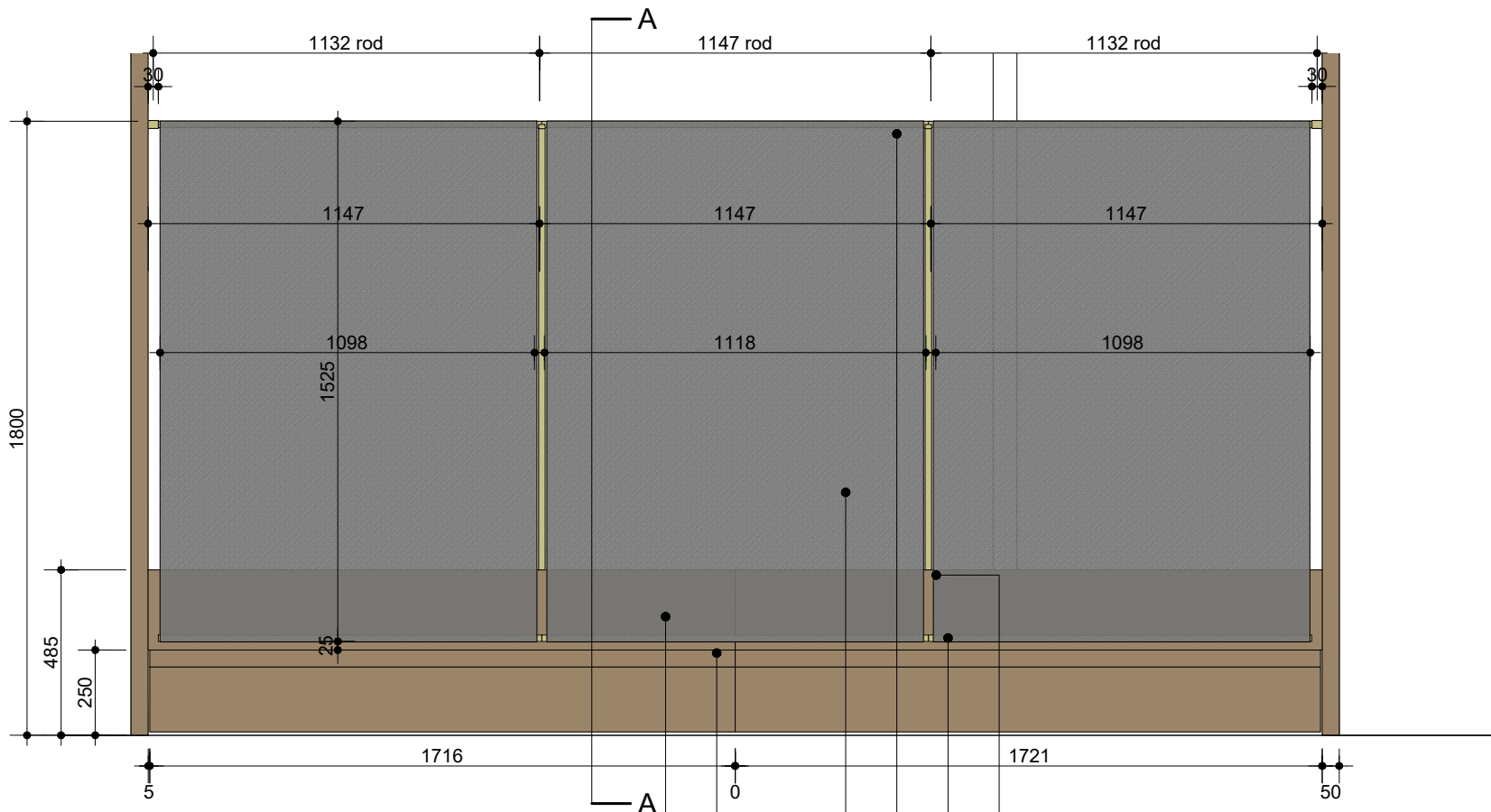
1 Elevation - Bay 1 - Fixed Scale 1:20
