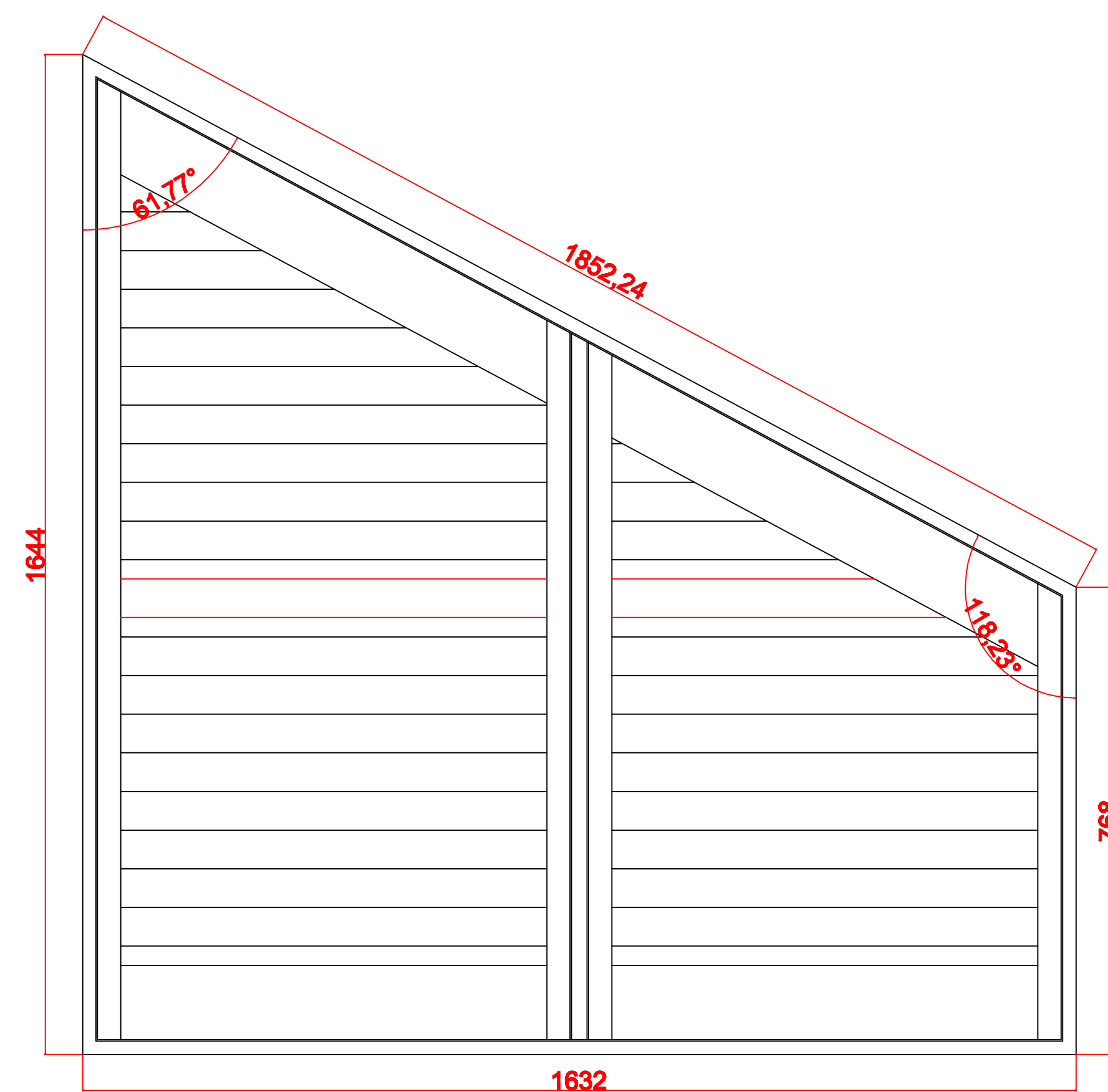
HP-4240-2-LTL Extra louvres *2
