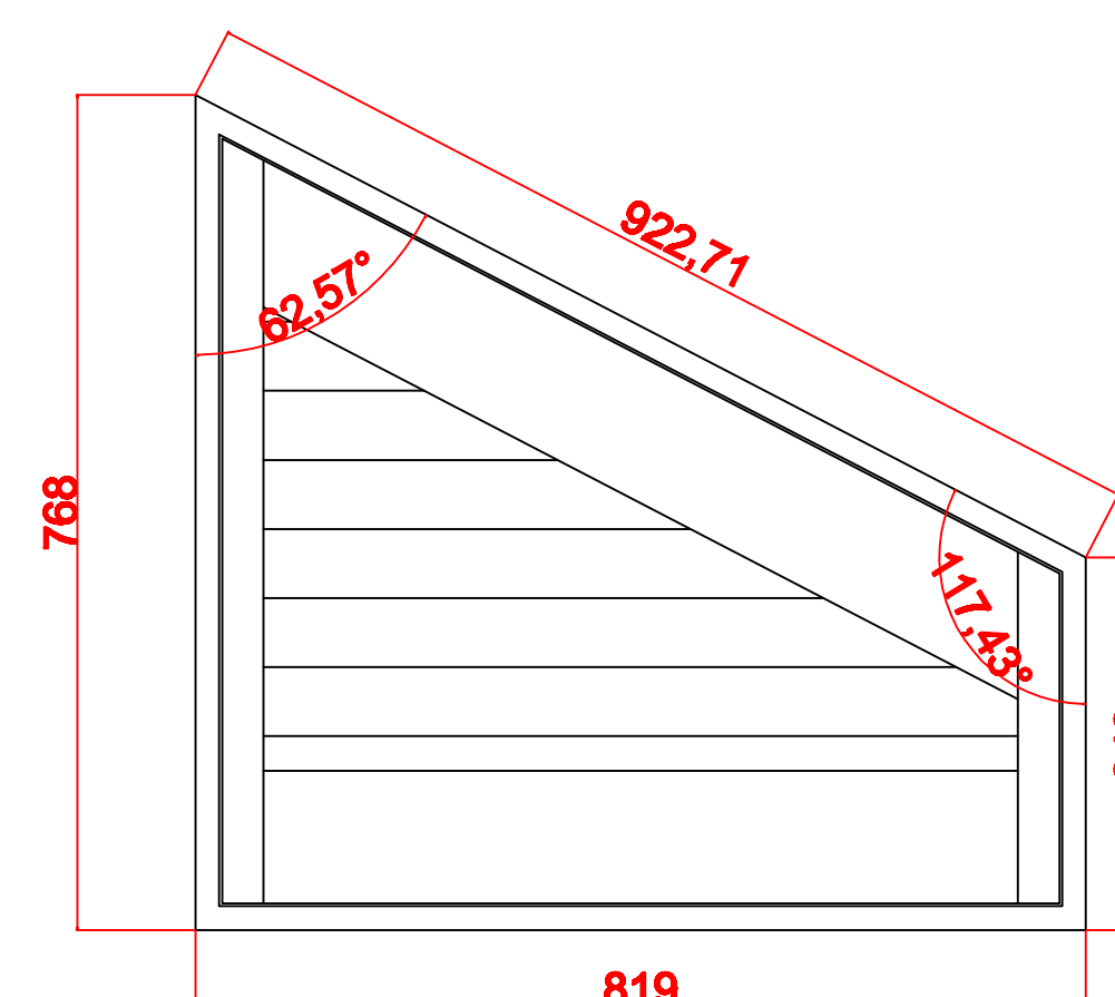
HP-4240-3-L Extra louvres *2
