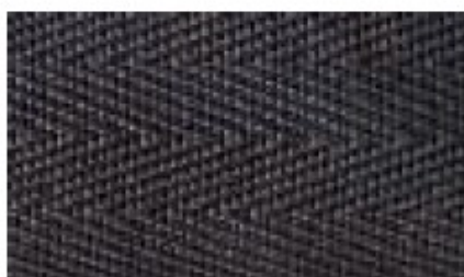
BASALT
