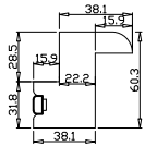
Deep BullNose Z Frame 38mm
