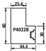
Frame: P4022B
