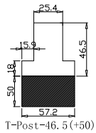
T-Post-46.5(+50)
