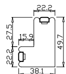
Double Insert L Frame 50mm
