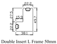
Double Insert L Frame 50mm
