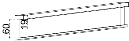
Frame (Left/Right) 左右边框: 60*19*1995m m *2
