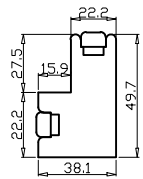
Double Insert L Frame 50mm
