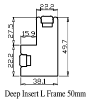
Deep Insert L Frame 50mm
