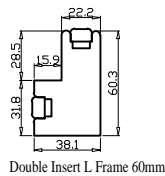
Double Insert L Frame 60mm
