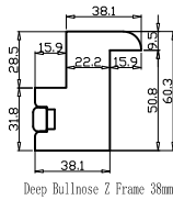
Deep Bullnose Z Frame 38mm
