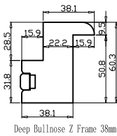
Deep Bullnose Z Frame 38mm
