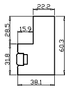
Z Sill Plate Top/Bottom/Right
