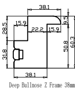
Deep BullNose Z Frame 38mm
