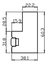
Z Sill Plate
