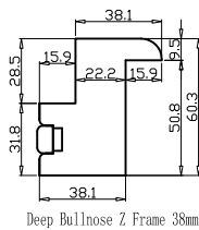
Deep Bullnose Z Frame 38mm
