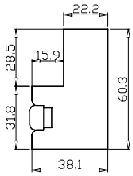
Deep Plain L Frame 6mm
