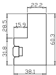
Deep Plain L Frame 60mm
