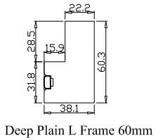
Deep Plain L Frame 60mm
