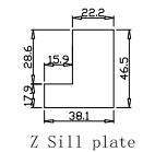
Z Sill plate
