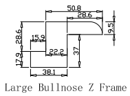
Large Bullnose Z Frame
