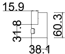
Z Sill Plate
