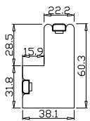
Double Insert L Frame 60mm
