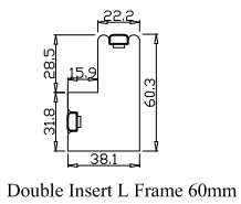
Double Insert L Frame 60mm
