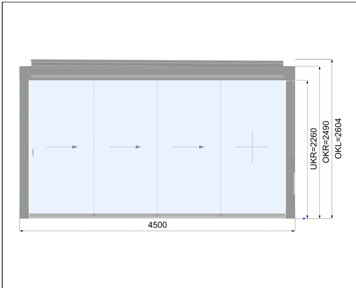
side view 3
