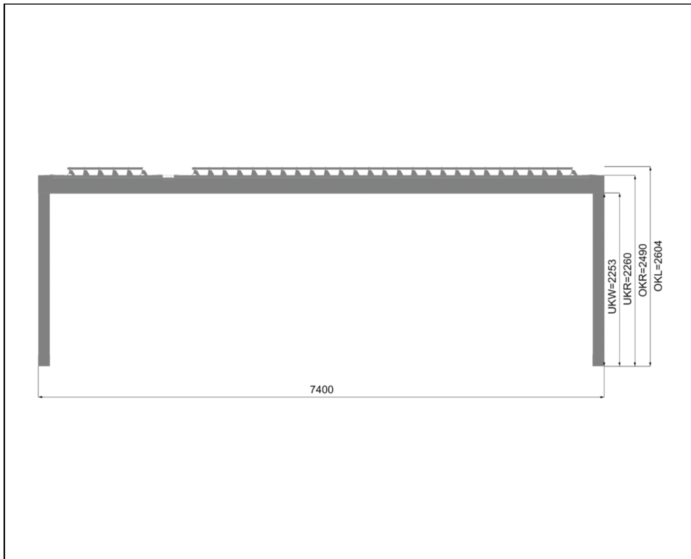
side view 4
