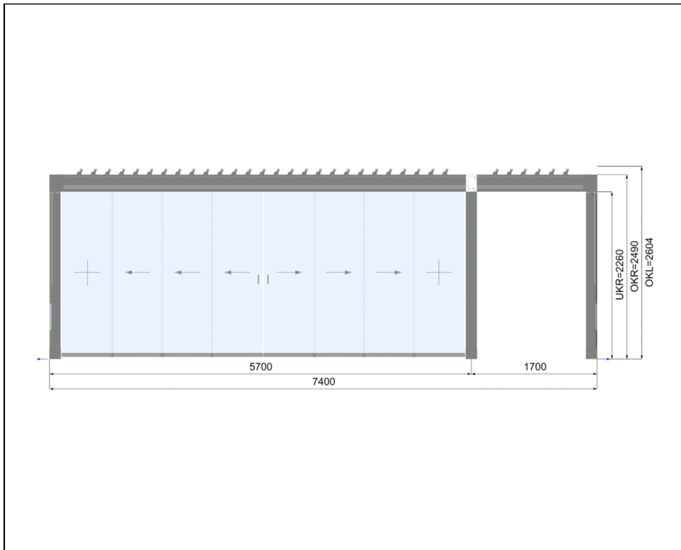
side view 2
