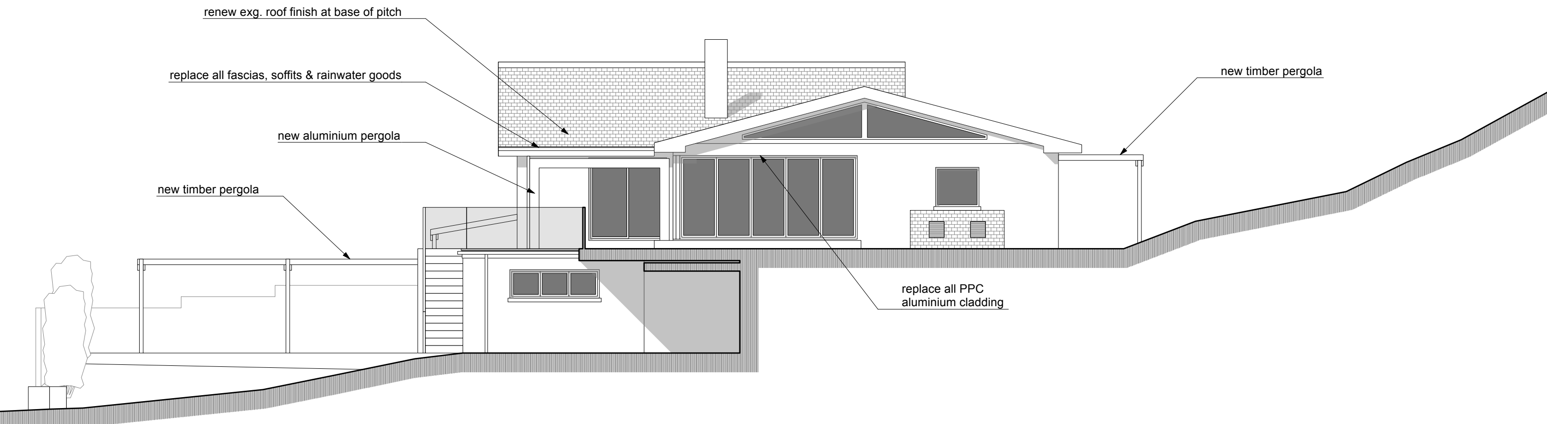
South-east elevation
