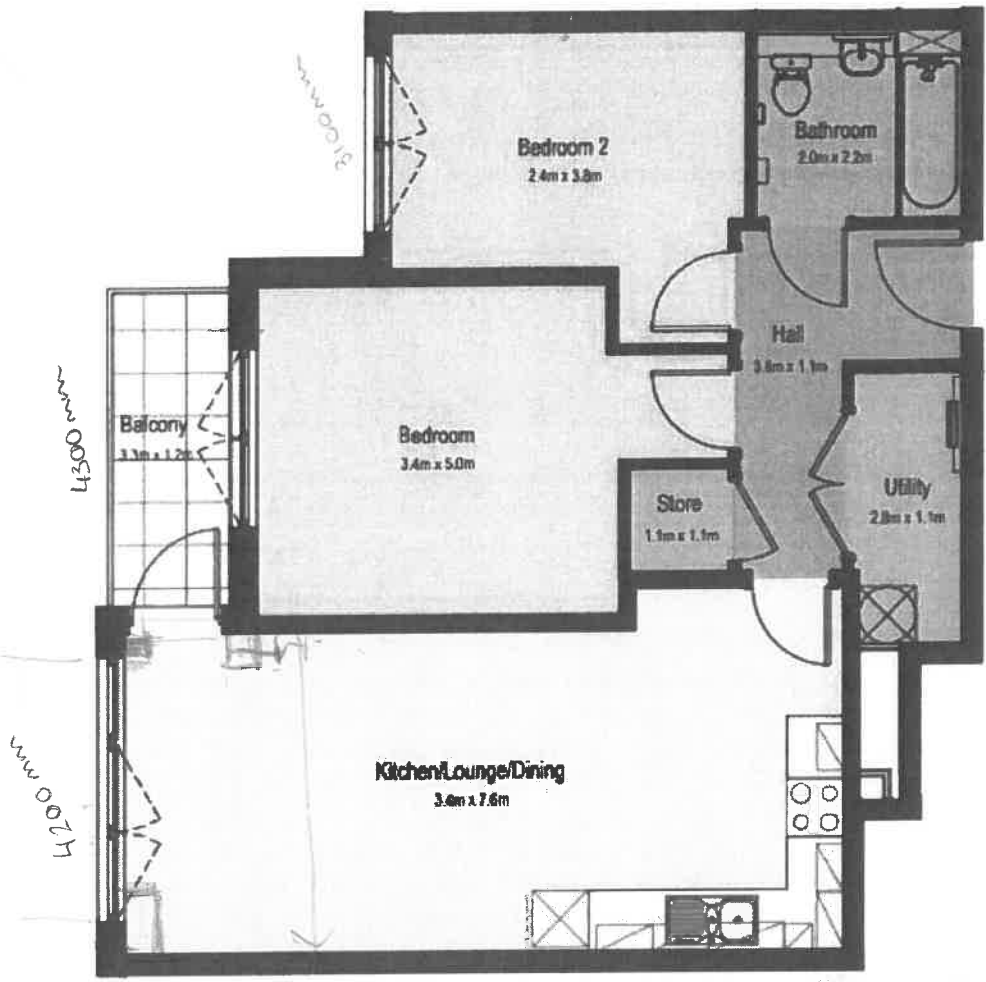
Key Plan - Block A - FOURTH FLOOR
