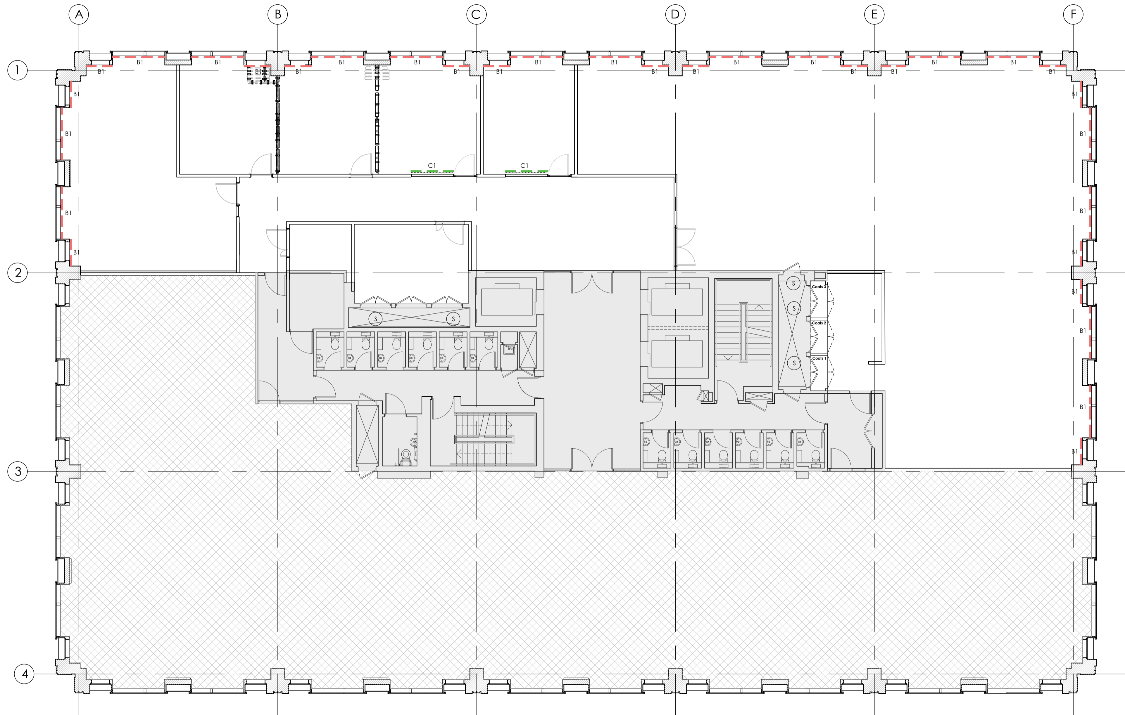
BLIND AND CURTAIN STRATEGY AS PROPOSED @ 1:100
