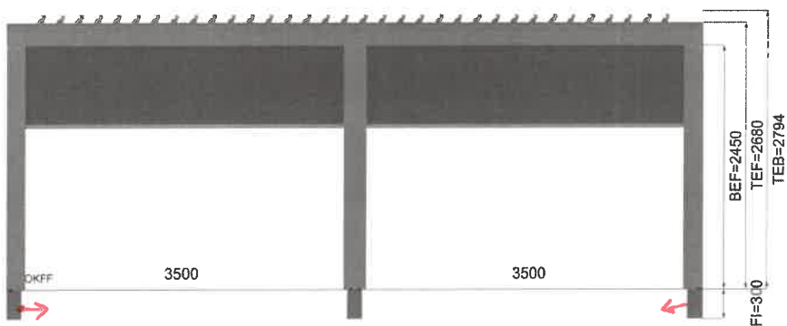
side view 2
