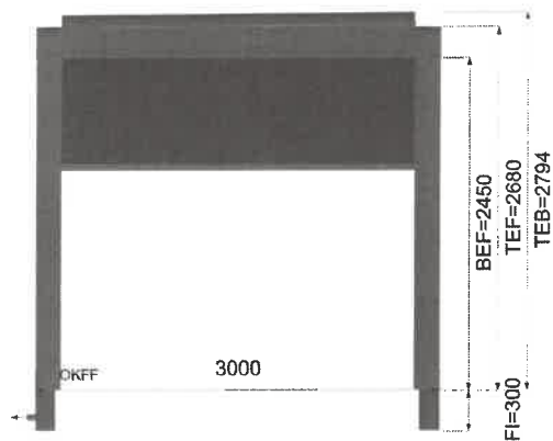
side view 2
