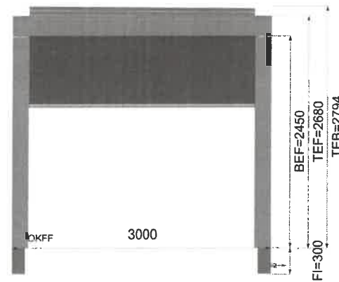
side view 4
