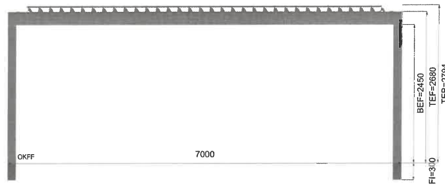
side view 4
