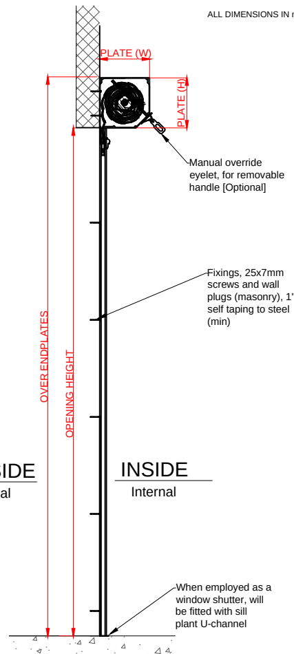
TYPICAL THROUGH SECTION
