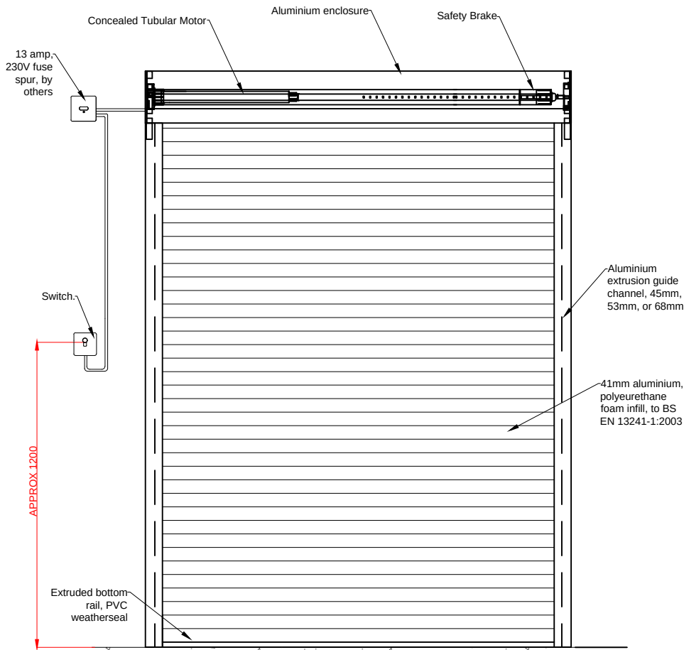
ELEVATION VIEWED FROM INSIDE
