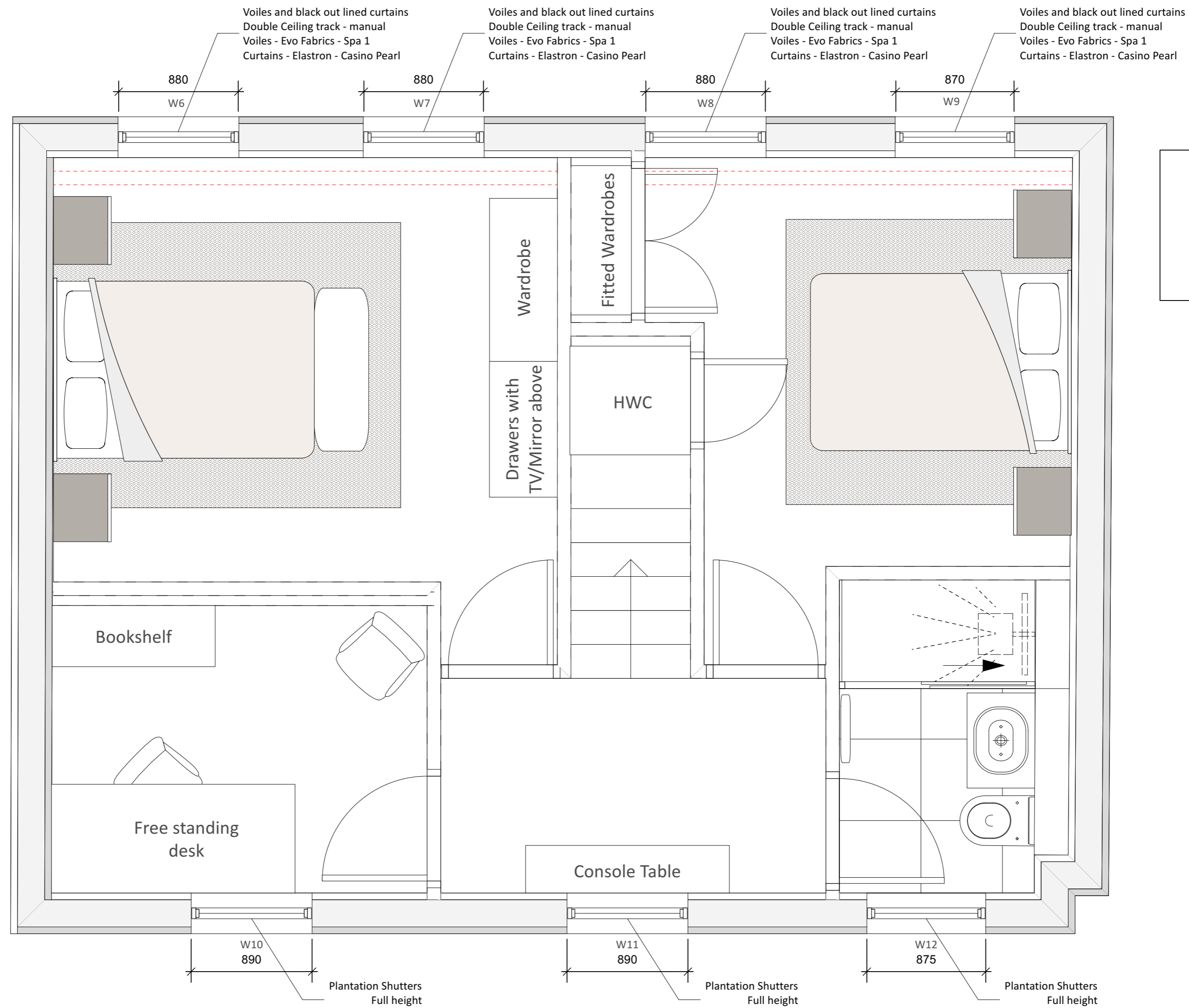
1 First Floor - Proposed Window Treatment Plan Scale: 1:25
