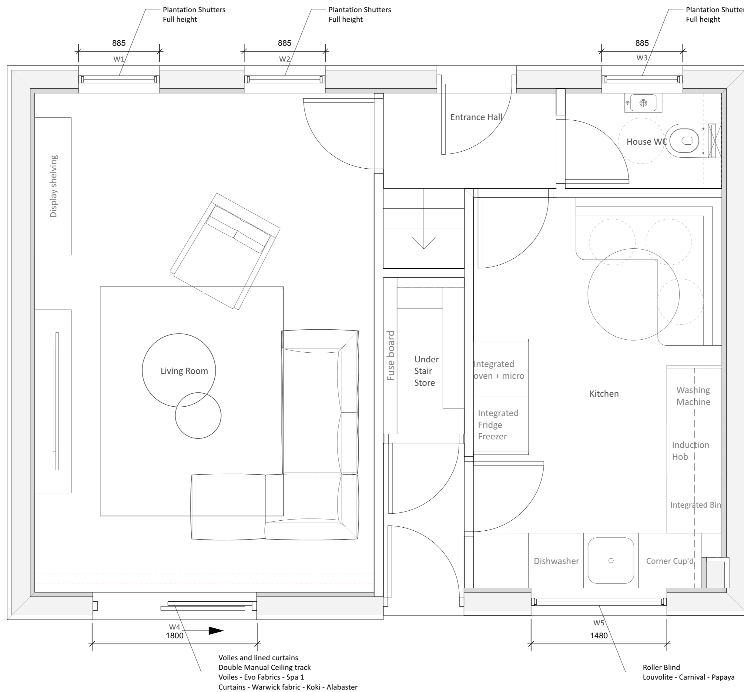
1 Ground Floor - Proposed Window Treatment Plan Scale: 1:25
