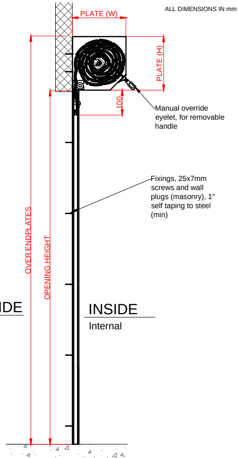
TYPICAL THROUGH SECTION
