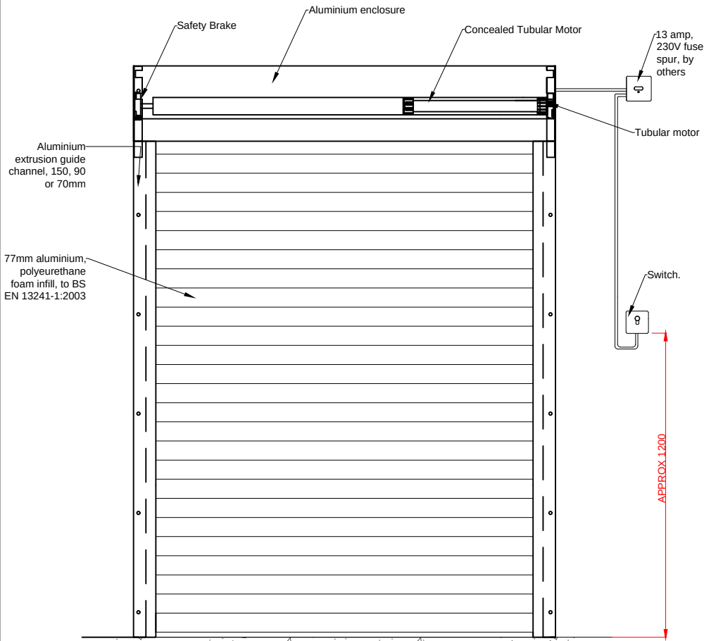
ELEVATION VIEWED FROM INSIDE
