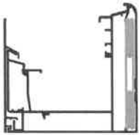
gutter cross-section
