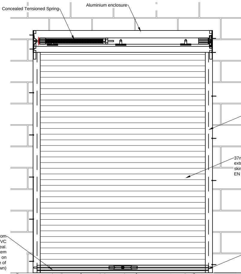
ELEVATION VIEWED FROM INSIDE
