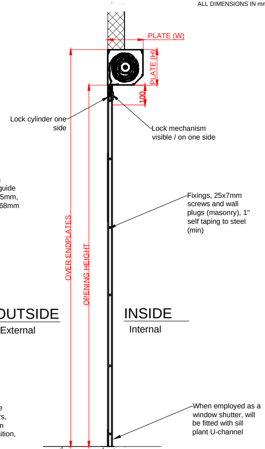
TYPICAL THROUGH SECTION
