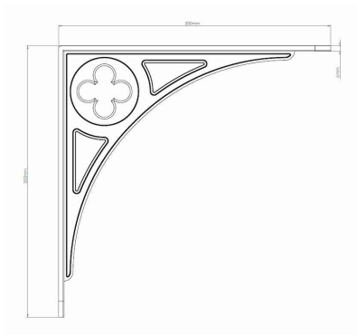
(300x300 Gallows Bracket)
