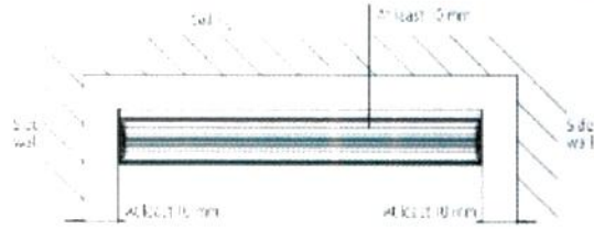
Side view of roller blind installation
