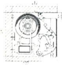
Top view of roller blind installation
