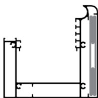
gutter cross-section
