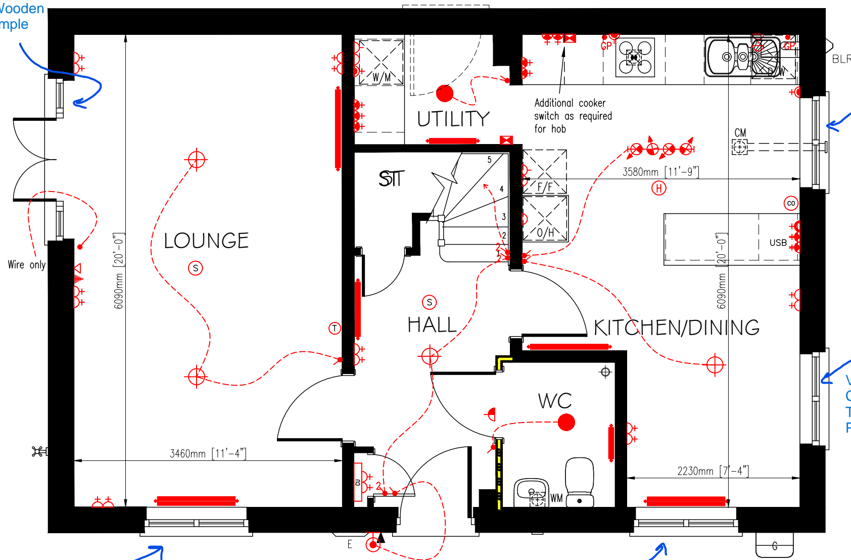
GROUND FLOOR PLAN (OPP)
