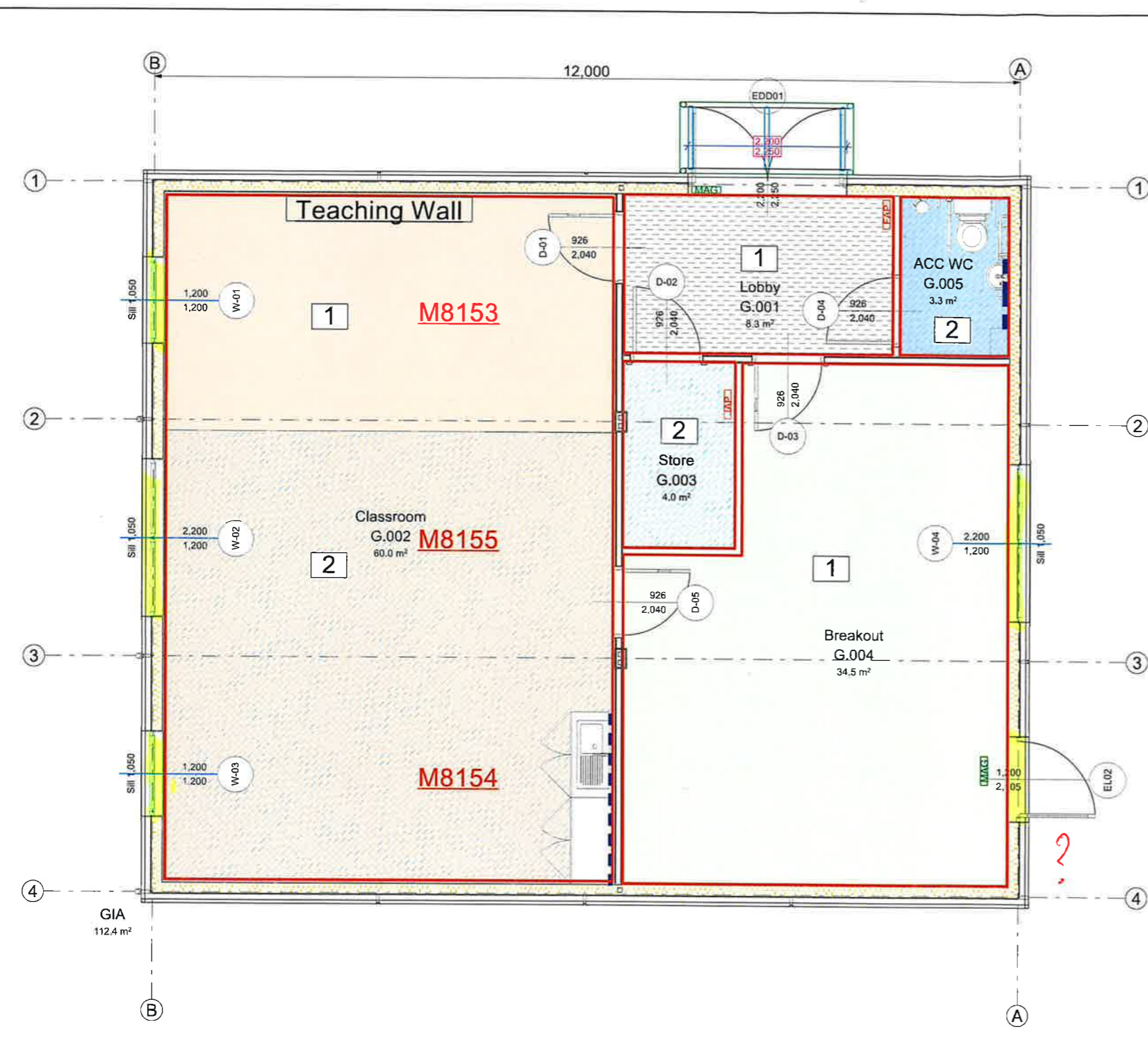
0. Ground floor Internal finishes 1:50
