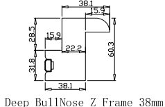
Deep BullNose Z Frame 38mm
