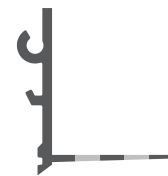
P - Perforated flange.
