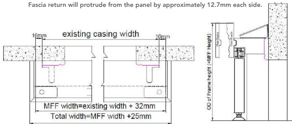
Top View (With existing casing)
