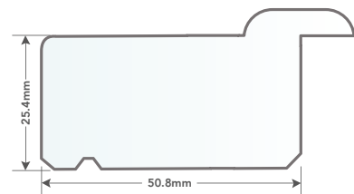
50mm D-Mould Stile
