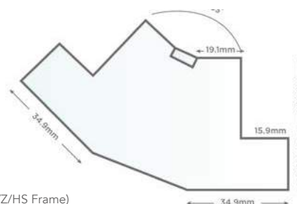
(L/Z/HS Frame) 46mm with insert
