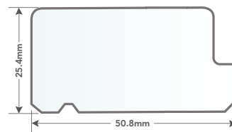
50mm Rebate Stile
