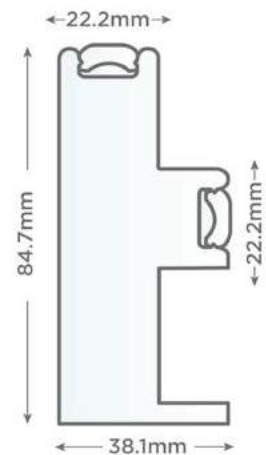
Double Insert F Frame 84mm
