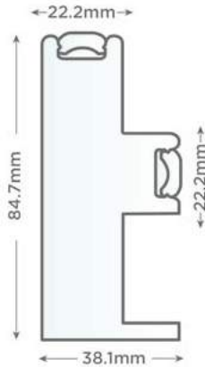
Double Insert F Frame 84mm
