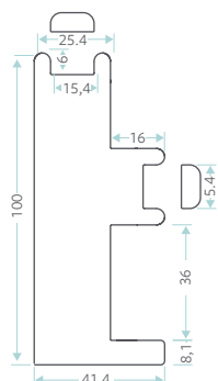
Blockout Frame 100mm
