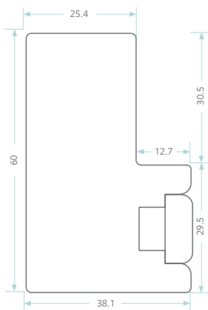
PVC Plain L Frame with Insert 60mm
