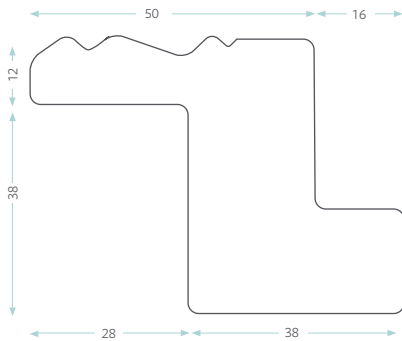
Regal Z Frame with Insert 76mm
