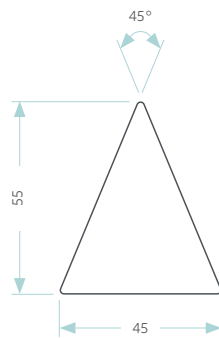
Triangle Batten for 135° Bay
