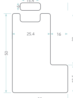
Vintage L Frame 50mm
