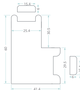
Vintage L Frame Double Insert 60mm
