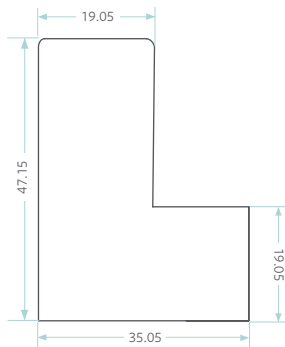
PVC Plain L Frame 50mm
