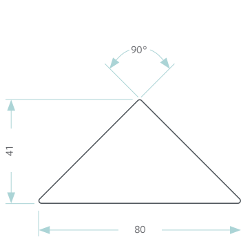
Triangle batten for 90° Corner
