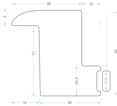
Regal Z Frame 76mm
