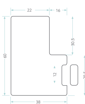
Plain L Frame 60mm
