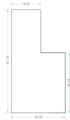
PVC Plain L Frame 70mm
