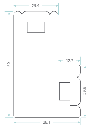
PVC Vintage L Frame with Double Insert 60mm
