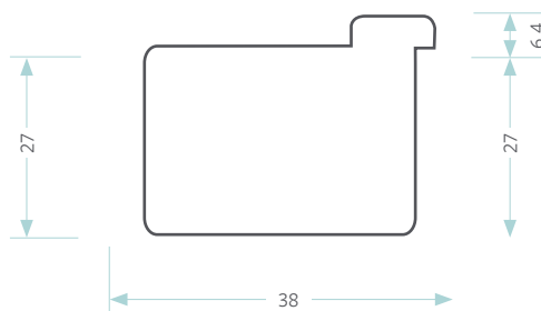
38MM BEADED RABBET STILE
