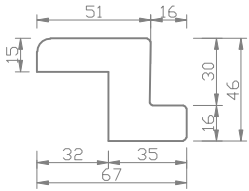
Large Z Classic (Z-50)
