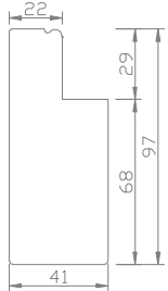
97mm Bead L-Frame
