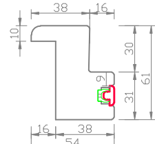
DEEP BULLNOSE Z FRAME
