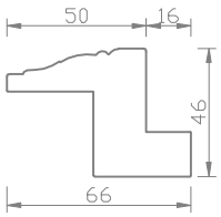
Std Trim(Colonial)
