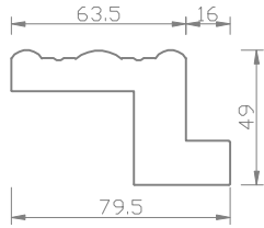
Fancy Z Trim
