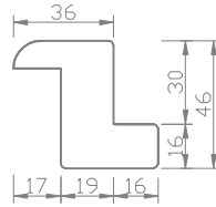
BullNose Z-Frame(Z38)
