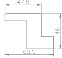
Plain Z Trim
