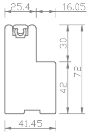
Pv Vintage L Frame 72mm
